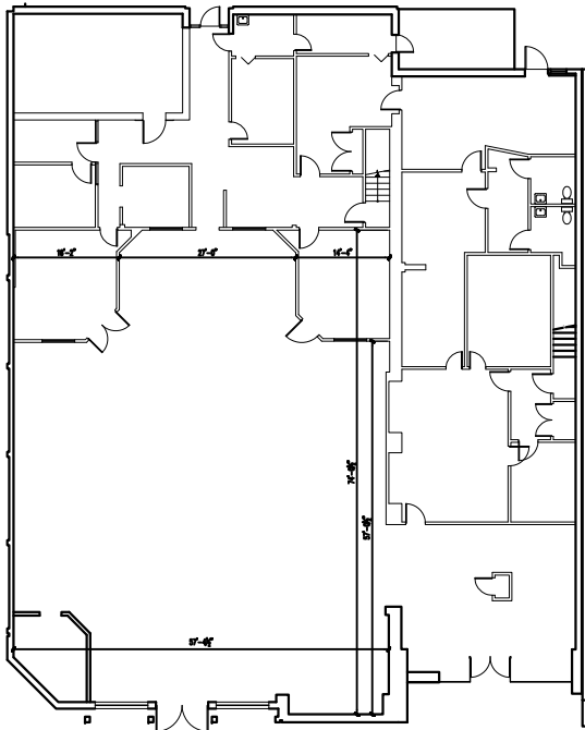
FLOOR 1 8,469 RSF SCALE: 1/32" = 1'-0"
